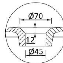
water drainer
