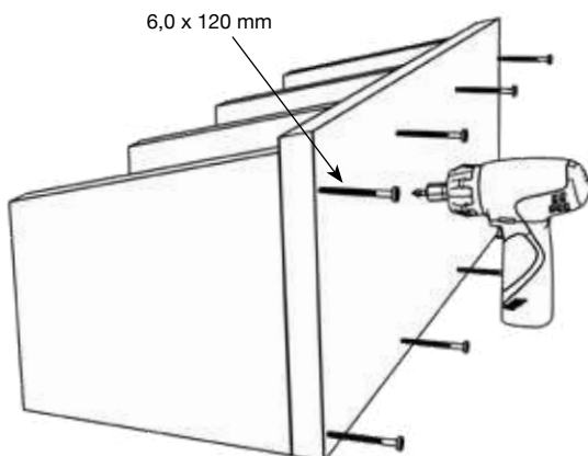
5) Bolt on supporting panels A.
