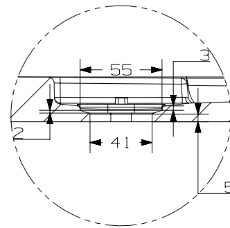
DETAIL C SCALE 0.286:1.0
